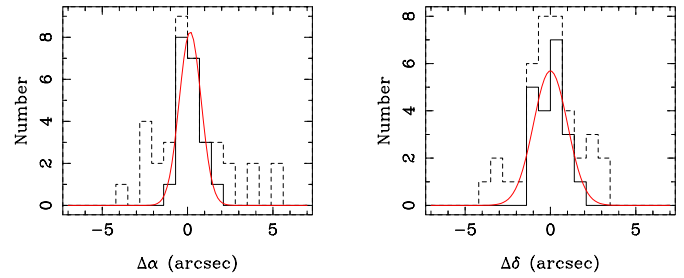
Fig. 2. Residual position differences between X-ray source positions and potential optical counterparts extracted from deep i CCD images obtained with the INT WFC (see section 5). The solid histogram shows the distribution for counterparts with a high likelihood of being the correct identification. The dashed histogram shows the distribution for all potential candidates. The red curves show the Gaussian fits to the solid histogram data points.
