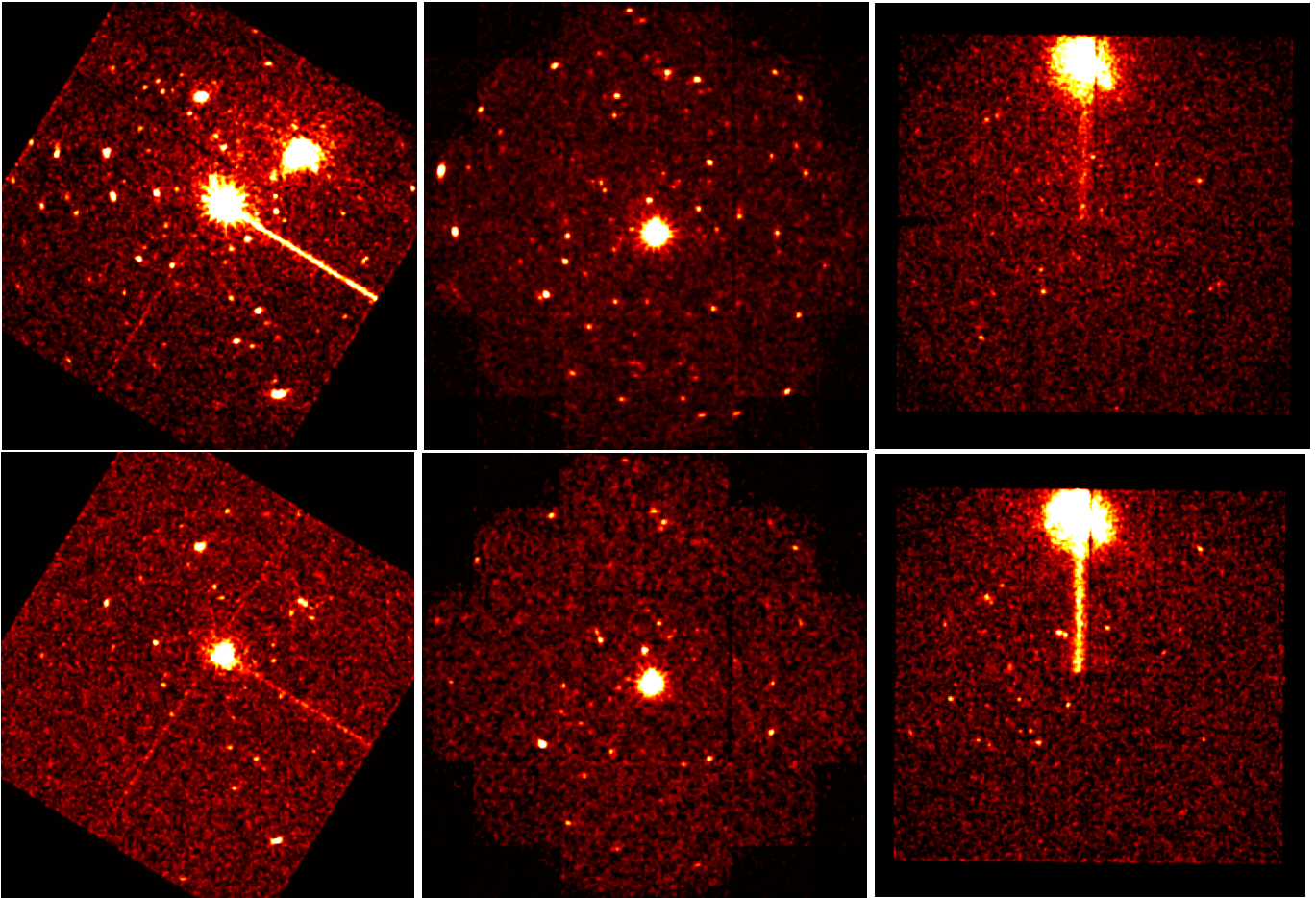
Fig. 1. EPIC images of three fields. Essentially the whole field, 30 arcmin. across, is shown in each case. Top row shows the soft band (0.5-2 keV) images and the bottom row the corresponding hard band (2-10 keV) images. Left: Mkn 205, EPIC pn image; Centre: OY Car, EPIC MOS1+MOS2 image; Right: G21.5–0.9 (offset pointing), EPIC pn image. Further details are given in Table 1. The images have been smoothed to aid the visibility of faint sources. The trails associated with bright sources in the pn images are due to ‘out-of-time’ events which arrive during the read-out cycle of the CCDs and have not been screened out.
