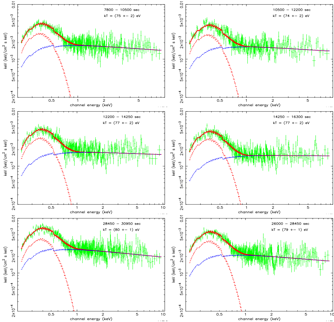
Fig. 7. Black body and power-law fit to the EPIC pn spectra of Mrk 766 for different time intervals. Upper two panels: Spectra selected for the high (left panel) and the low (right panel) flux state for the periodicity peak centered at 9000 seconds (corresponding to the time given in Figure 1.) The temperature of the black body component remains constant within the errors. Middle and lower panels: Same as above for the periodicity peaks centered at 13220 and 29700 seconds.
