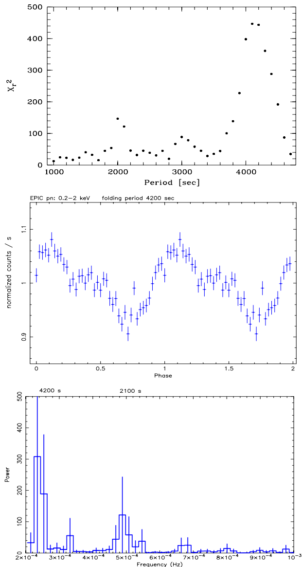
Fig. 2. Upper panel: Reduced \chi_r^2 versus the folding period for the 0.2–10 keV energy range. Middle panel: Folded 0.2–2 keV light curve with the best fitting period of 4200 seconds. Lower panel: Power spectrum for Mrk 766 in the 0.2–10 keV energy band.
