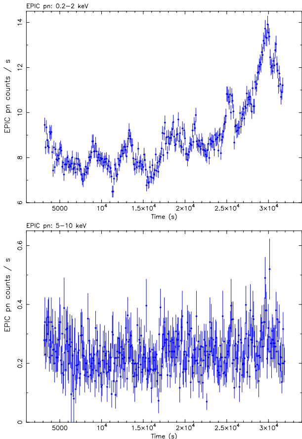
Fig. 1. XMM Newton EPIC pn light curve of Mrk 766 in the 0.2–2 and 5–10 keV energy band, respectively.
