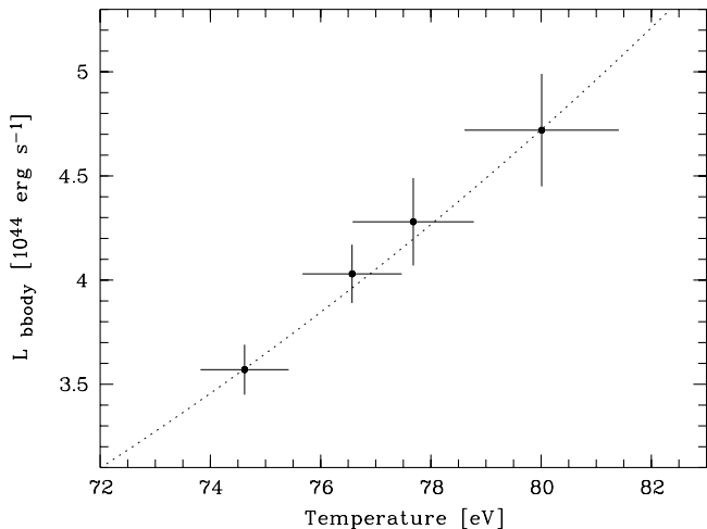
Fig. 8. Black body temperature versus the bolometric black body luminosity for 4 different time intervals selected from the light curve shown in Figure 1. The temperature increases with the source luminosity according to a black body emission law.
