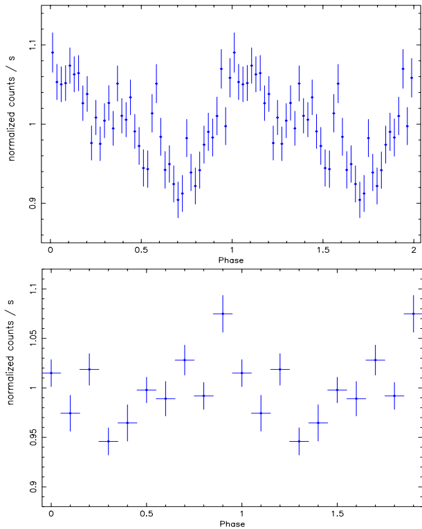
Fig. 3. Folded MOS-1 light (upper panel) and RGS-1 light (lower panel) curves using the best fitting period of 4200 seconds. The folded RGS light curve covers a longer time scale compared to the EPIC data, therefore both light curves are not in phase.
