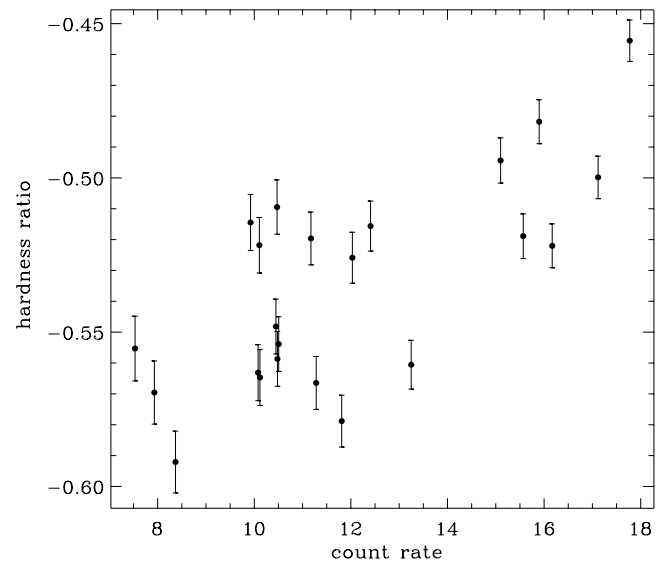
Fig. 2. Hardness ratio (hard-soft)/(hard+soft) versus total count rate. Every data point corresponds to 2000 s integration time. Soft band (0.2-1 keV), hard band (1-10 keV).
