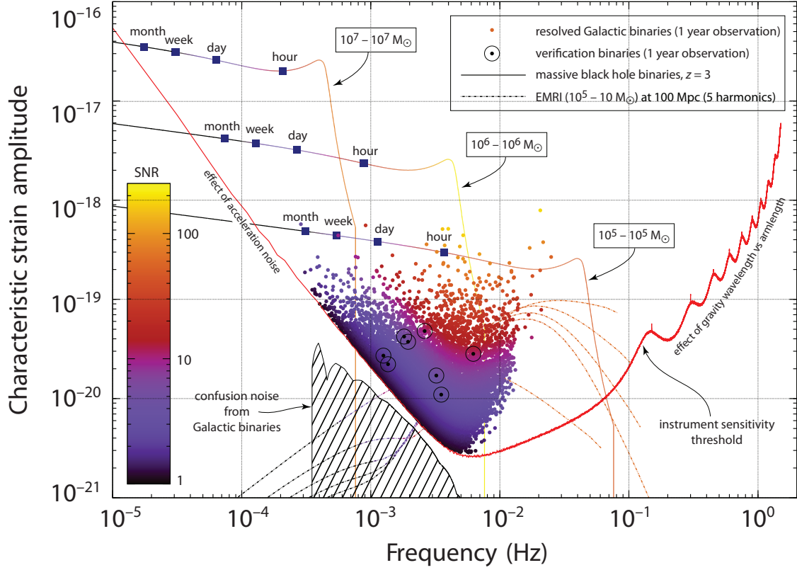
Figure 2.1: Characteristic strain amplitude, \sqrt{h(v)} , versus frequency for a space-based laser interferometry mission (armlength = 1 \times 10^6 km, 1-yr observations). Objects expected to be strong gravitational wave sources over this frequency range are indicated. For compact white dwarf binaries, individual simulated sources, known ‘verification binaries’, and the effect of confusion noise from the ensemble of fainter sources, are shown. Dashed lines give example loci for extreme mass ratio inspirals (EMRIs) for the case of a 10^5 M_\odot - 10 M_\odot binary (and showing the 5 strongest harmonics). Solid curves show three example loci of massive black hole binaries of different mass, labelled with the time intervals over which the source remains ‘in band’. In all cases, colour coding shows the corresponding (cumulative) S/N, increasing toward higher frequency as each system becomes more compact (this version courtesy Stas Babak, AEI, and Antoine Petiteau, APC).
