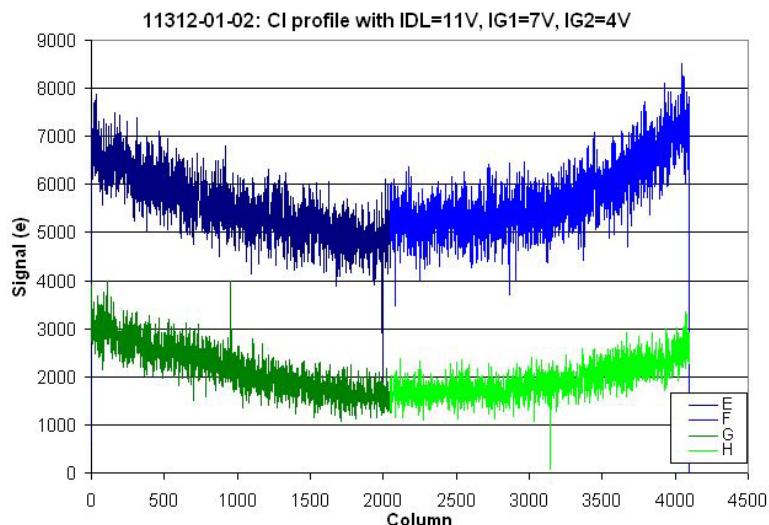
Figure 4 shows two row profiles of injected signal for a front illuminated CCD273-84.
