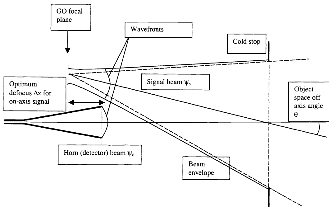
Figure.1. Beam geometry for calculation of efficiency.
