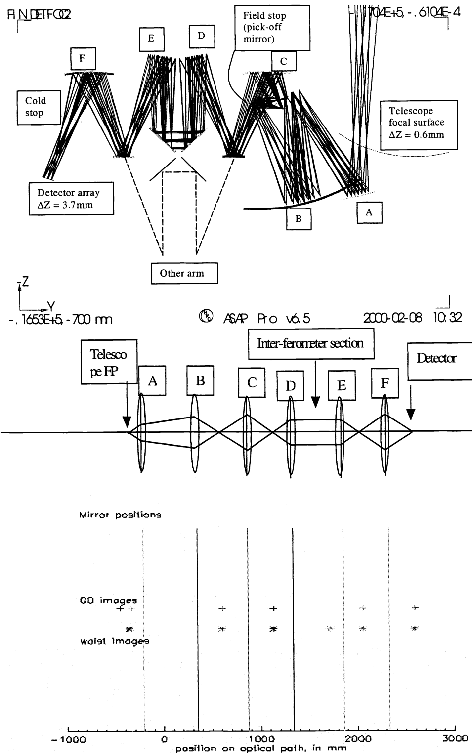
Figure 2. FTS optics ray-trace, equivalent unfolded imaging system, and plot of image positions, for case \lambda=0.5\text{mm} . The input beam waist is positioned co-incident with the GO focus of the telescope primary mirror, and its offset from GO focus at subsequent focal planes is labeled \Delta z in the ray-trace.
