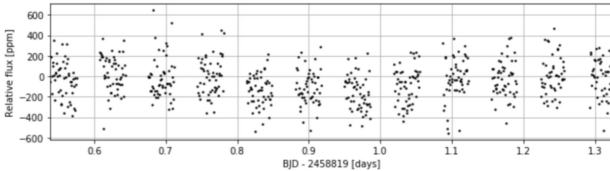
Figure 21: Case 2. A Sun-like star (G2V, 5770 K) of V=9 transited by an Earth-size planet with an orbital period of 50 days. Basically, this is the same case as in Figure 20 albeit with a fainter target. The exposure time is 10 s and on-board stacks contain 6 images.
