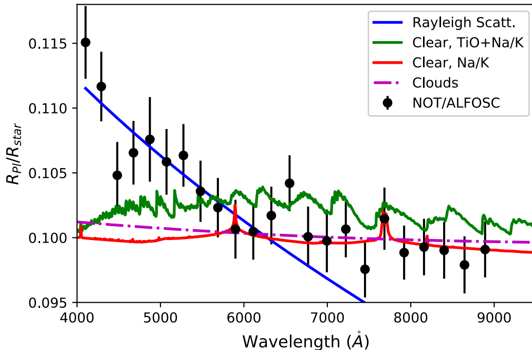
Transmission spectrum. WASP-74b
