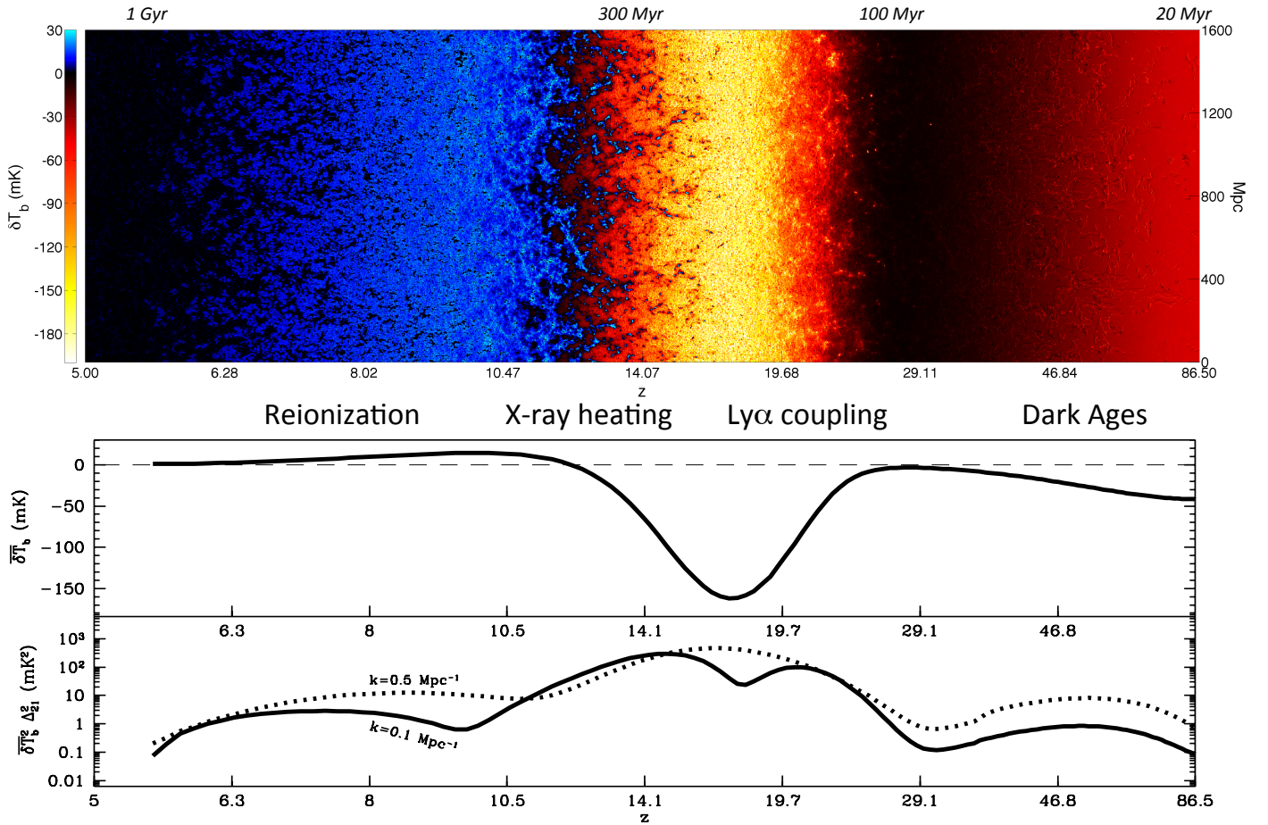
Fig.1: 2D slice through a mock 21-cm lightcone (top), corresponding global global signal evolution (middle), and the 3D power spectra at two wave numbers (bottom). Some major cosmic milestones can be seen from right to left: (i) Wouthuysen-Field (or Lyman- \alpha ) coupling (Wouthuysen 1952, Field 1959), when Lyman-band photons efficiently couple the spin temperature to the gas temperature (black to yellow); (ii) epoch of heating, when galactic X-rays with long mean free paths heat the predominantly neutral IGM (yellow to blue); (iii) epoch of Reionization, when ionising photons drive the final major phase transition of our Universe (blue to black). The timing and the patterns of the signal encode a wealth of information about the first galaxies. This figure corresponds to the fiducial model of Mesinger et al. (2016), though recent studies calibrated to high- z galaxy observations suggest that the Cosmic Dawn epochs of WF coupling and X-ray heating might occur later, with significant overlap with the EoR, due to less efficient star formation (e.g. Park et al. 2019).
