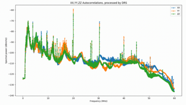
Fig.7: First data taken during an end-to-end test in January 2019. The different colours represent the autocorrelations from the 3 antenna units. On top of the broad band variations, with represent the variations in the response, there are clear sharp noise peaks most likely coming from electronic systems on the spacecraft.
