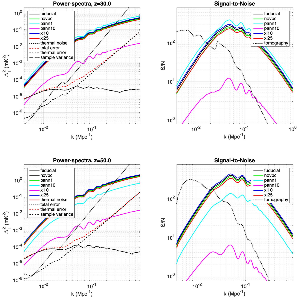
Fig 8. Top Left: Simulated power spectra of the 21-cm line based on Ali-Haïmoud, et al. (2014); Chen et al. (2016) (top solid solid lines; the fiducial model is in black (the top four power spectra are offset by 10% for clarity) and the expected sensitivity of the DEX array (red dashed line) for z=30 for a 10 \text{ km}^2 core and a 5-year mission, using a \text{BW}=10\text{MHz} . Top Right: Signal-to-noise achieved. Bottom Left/Right: Idem for z=50 with a 100 \text{ km}^2 core. In both cases, the dotted line indicated the thermal-noise power-spectrum. In case the 21-cm signal exceeds the noise power spectrum, direct imaging of those scales (tomography) can be done. We note that direct imaging on the largest scales is not affected by sample variance and can typically be done for scales larger than half a degree ( k \sim 0.1 ).
