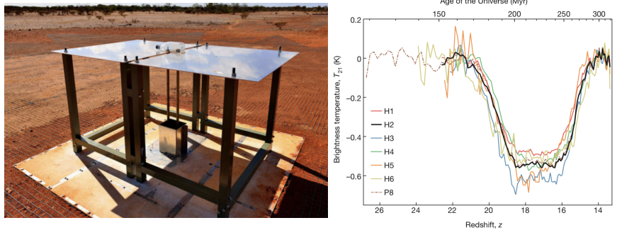
Fig. 4: The EDGES instrument (left) and its claimed global 21-cm signal detection (right)
