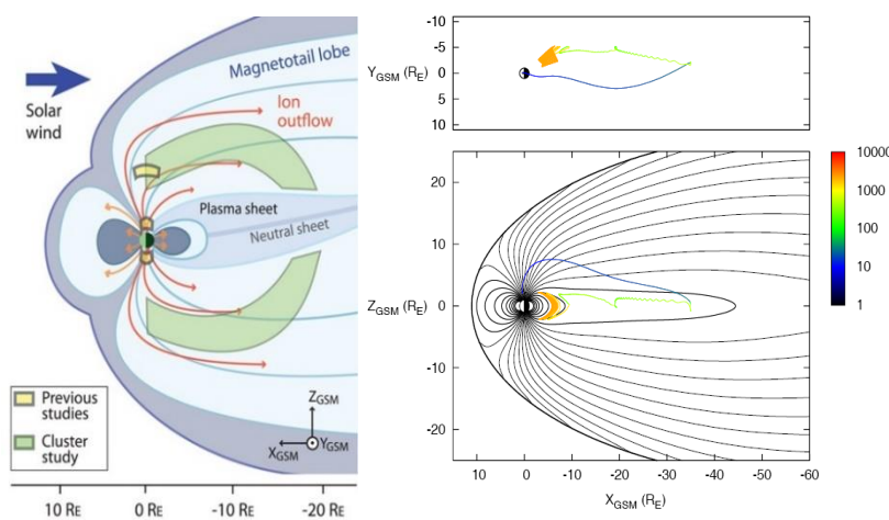
Figure 7. Schematic of “cold hidden” H + ion outflow in the magnetosphere, regions of existing satellite observations, and nominal PCW orbit (purple eclipse) (adapted from Engwall et al., 2009) (b) Typical trajectory of an O + ion originating from the cleft ionosphere as it transits the magnetosphere (after Howarth and Yau 2008)
