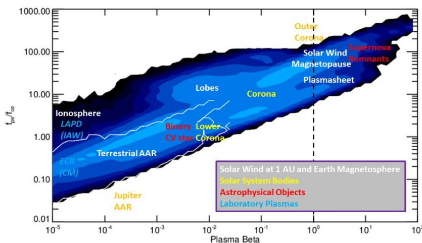
Figure 4. Properties of various solar system, astrophysical objects, and lab plasma regimes as a function of plasma frequency ( f_{pe} ), electron gyrofrequency ( f_{ce} ) and plasma beta ( \beta ). In colour are real measurements from the Cluster spacecraft over the lifetime of the mission, superimposed on this are regimes of each solar system, lab plasma or astrophysical object.
