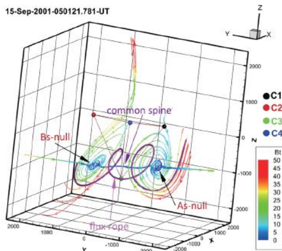
Figure 3. Magnetic field reconstruction results for a flux rope event showing a separator connecting a pair of A-B null points (after, Guo et al., 2016) and the limitation of a small spacecraft array for multiple structure.
