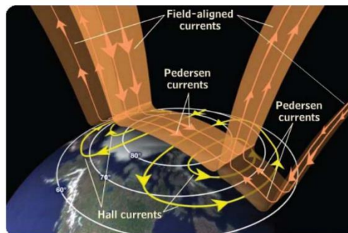
Figure 5. Magnetospheric current systems, linked via field-aligned currents (left) Coxon et al. (2014) and (right) COMET program, UCAR
