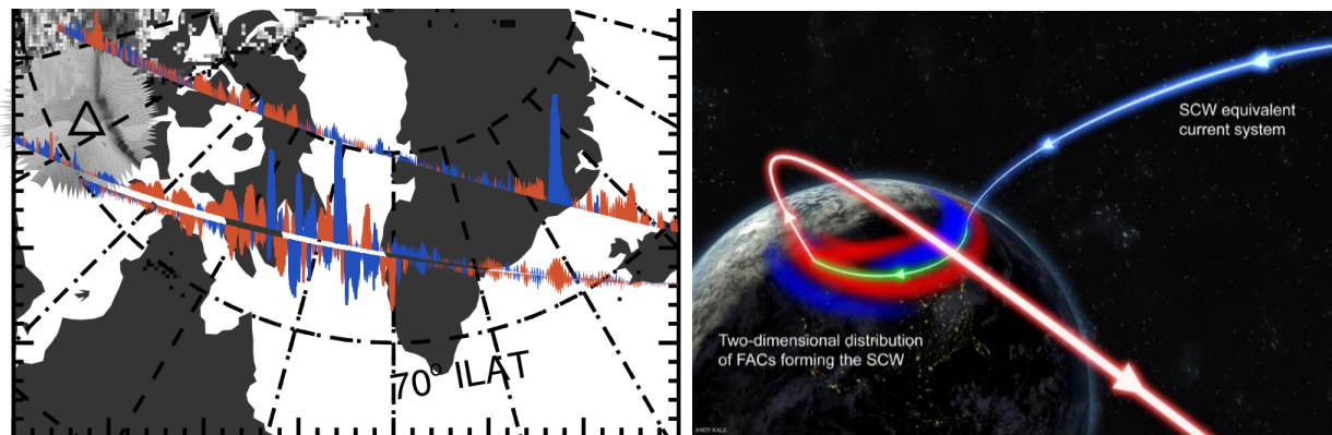
Figure 6. (left) Cluster observations of the spatial scales of FACs in the nightside magnetosphere-ionosphere; blue denoting FACs directed towards the ionosphere and red denoting FACs directed away from the ionosphere, together with (right) a schematic representation of the FAC structure on fluid scales
