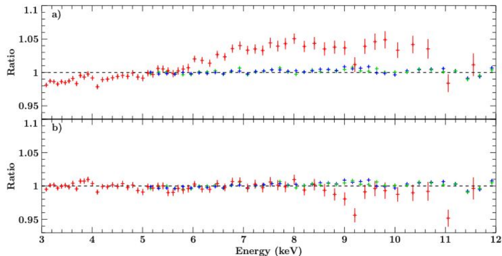
Figure 2: Stacked EPIC-pn (red) residuals, FPMA (blue), and FPMB (green) residuals of a joint fit to all Crab epochs, requiring the same photon index for all instrument in each epoch. a) Without any correction function for EPIC-pn. b) After applying the spline correction function.
