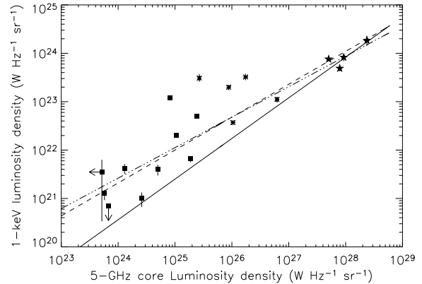
Figure 1. Luminosity-Luminosity relation. Filled boxes are RGs, asterisks are LDQs and star CDQs. Errors bars show 1\sigma uncertainties. When these are not visible it is because errors are smaller than symbols. Upper limits are at the 3\sigma level. The continuous line is the best-fit regression to the sample of CDQs only. The dot-dashed line is the regression to the whole sample, while the dashed line fits the sample composed of CDQs and RGs
