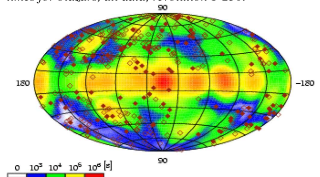
Figure 2. The IBIS INTEGRAL telescope total exposure times for blazars, all data, revolution 1-250.
