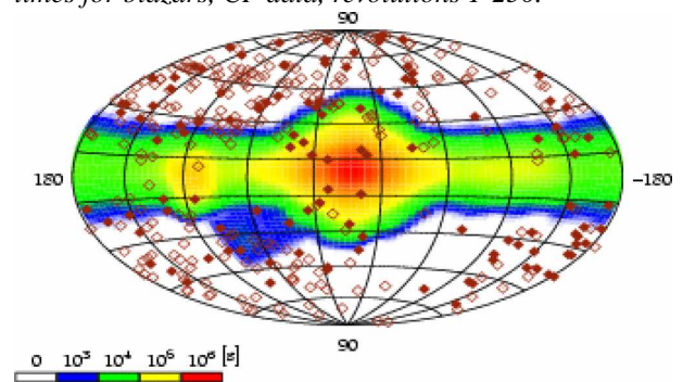
Figure 1. The IBIS INTEGRAL telescope total exposure times for blazars, CP data, revolutions 1-250.
