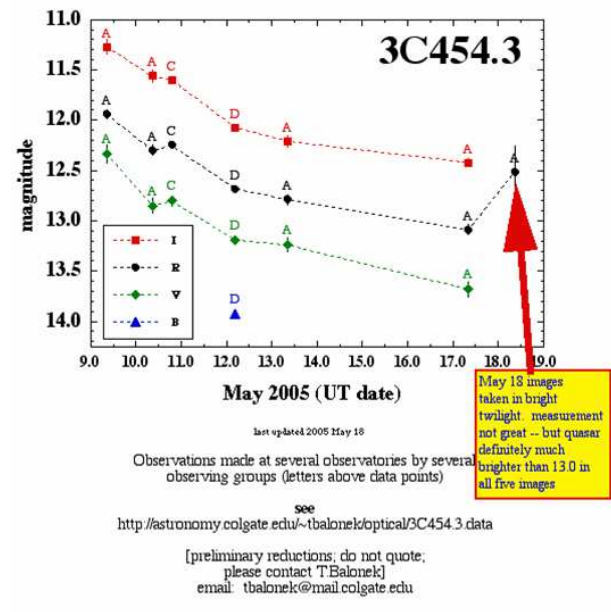
Figure 3. The optical light curve of 3C454.3 around the time of the INTEGRAL AO-3 ToO observation
