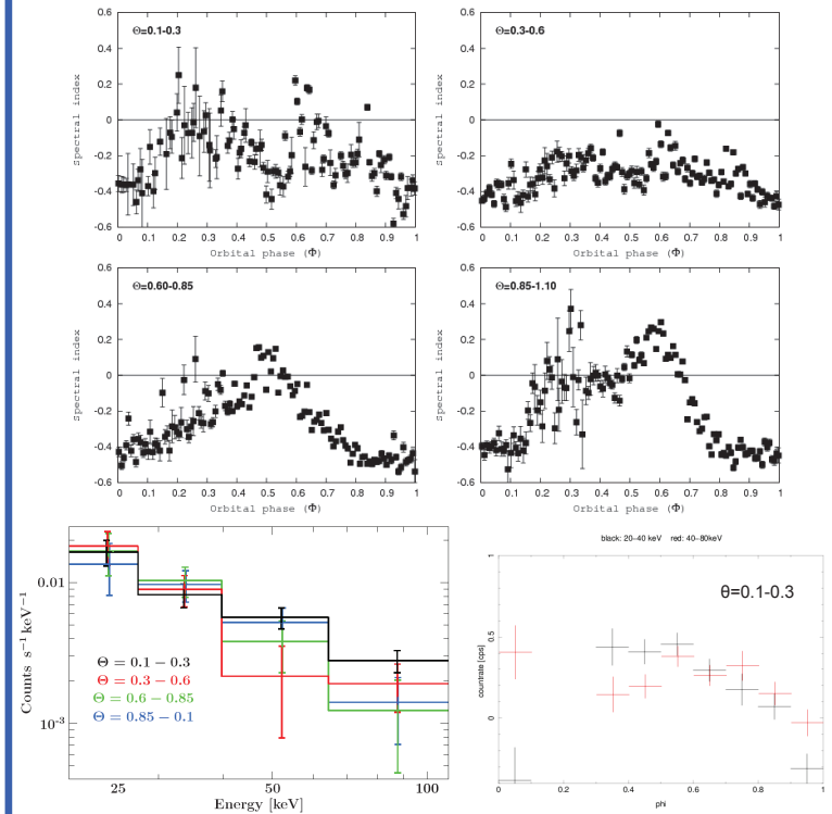
Fig.2 Top four panels: Radio spectral index ( \alpha ) evolution for LSI+61°303 along the orbit for four different \Theta intervals (according to the ephemeris of Gregory, P. C. 2002, ApJ, 575) calculated for 6.7yr data taken with the Green Bank Interferometer (Zimmermann, L., Grinberg, V. et al., work in progress).
