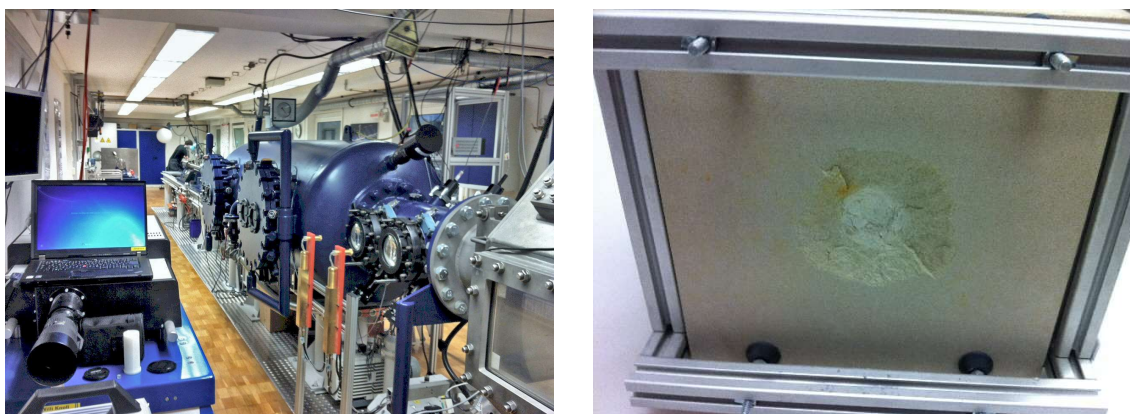
Fig. 9: Hypervelocity gas gun and target block of asteroid analog material, Fraunhofer Ernst Mach Institute, Freiburg, Germany. Credit: Alan Harris, NEOShield
