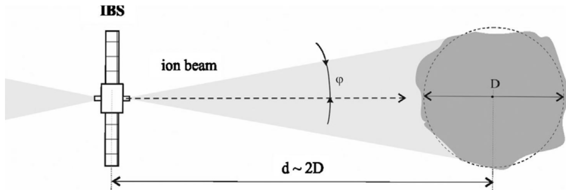
Fig. 10: Schematic diagram of the principle of the “ion-beam shepherd” deflection concept. A collimated beam of quasi-neutral plasma is directed at the asteroid surface. The spacecraft, placed at a distance of a few asteroid diameters, would need a second propulsion system to compensate for the ion engine reaction and keep a constant distance between the asteroid and the shepherd spacecraft. From Bombardelli et al., (2013).
