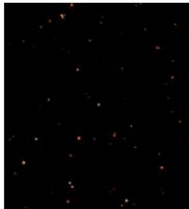
Groombridge 1830, 9.2 pc
