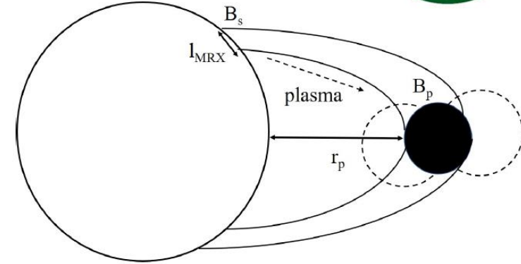
Magnetic field structure of close-by star – planet system.
